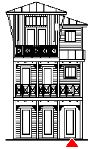
ELEVATION C
